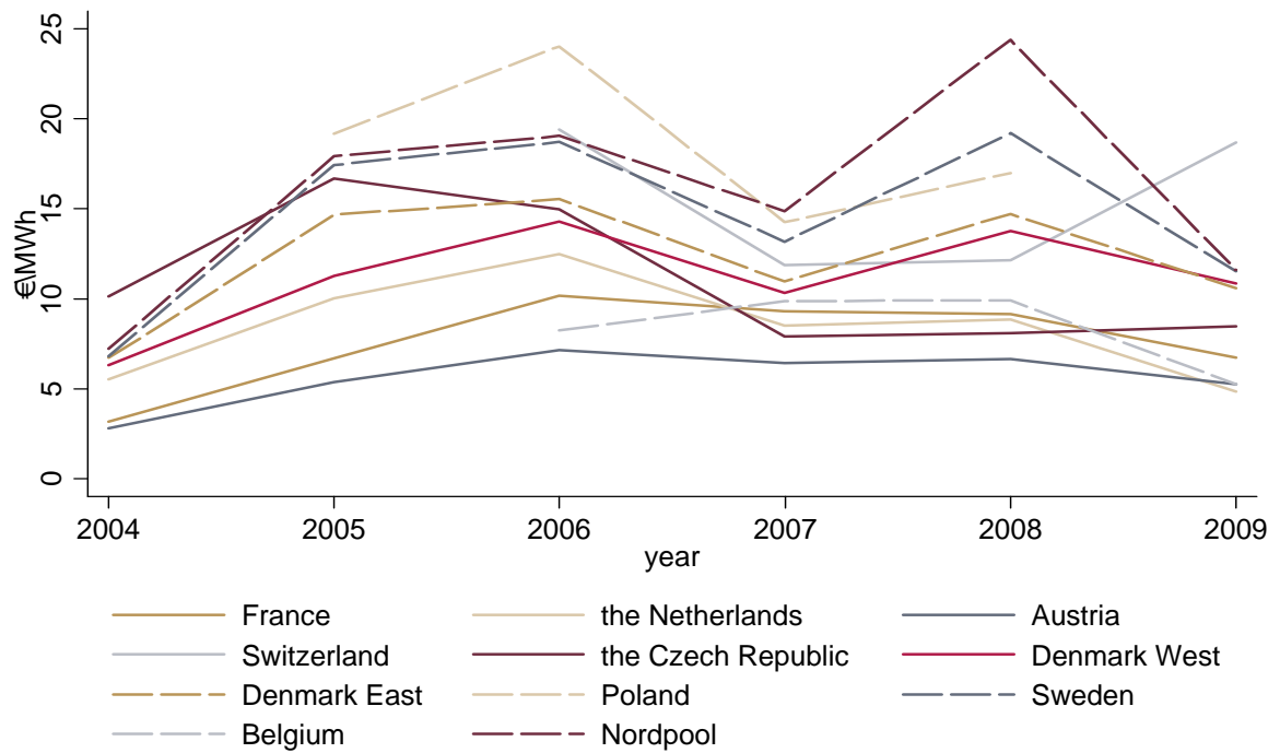
Figure 12: Absolute annually averaged day-ahead spot exchange market price differences
