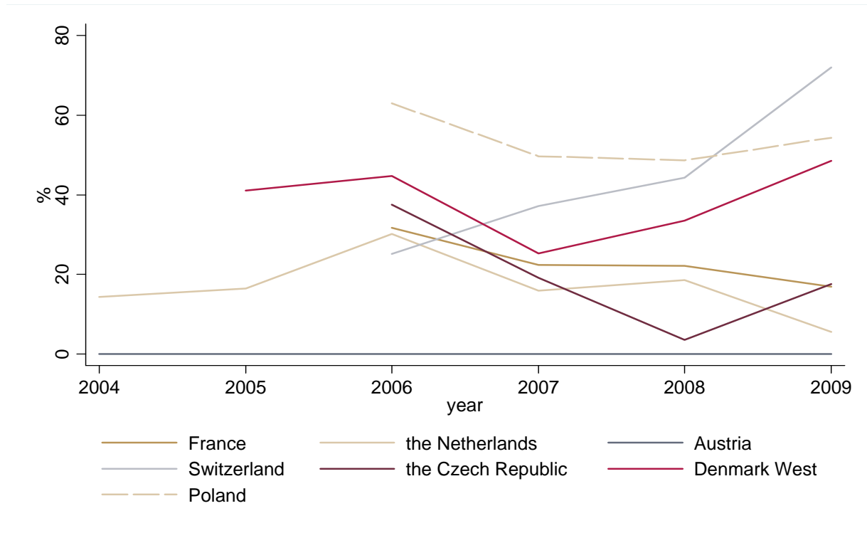
Figure 14: Share of hours in which interconnection price exceeds 10% of the German day-ahead spot exchange market price
